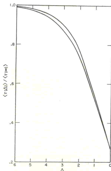
FIG. 21. Normalized scattering time vs \Delta for S=2.8 . The upper curve is the numerical calculation. The lower curve is the analytical approximation.
