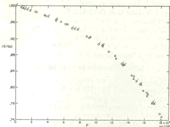
FIG. 6. Normalized conductance vs pressure for n -type germanium at 311°K for three samples. Points without ears were taken on increasing the pressure, those with ears on decreasing the pressure.
