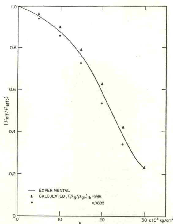
FIG. 17. Normalized effective mobility vs pressure for n -type germanium at 349°K.
